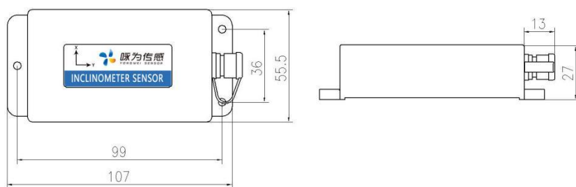
产品尺寸 L107*W55.5*H27mm
